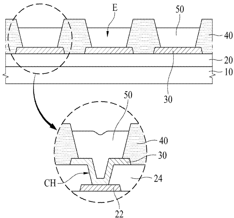
FIG. 1 RELATED ART
